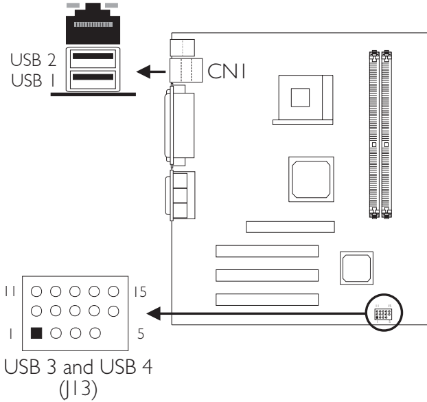
Additional USB Ports (USB 3 and USB 4)
