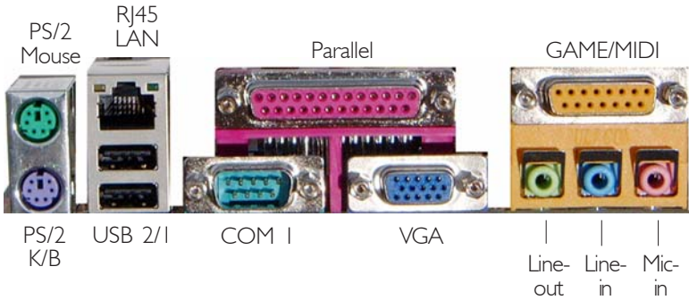
The Rear Panel I/O Ports on PM12-TL
